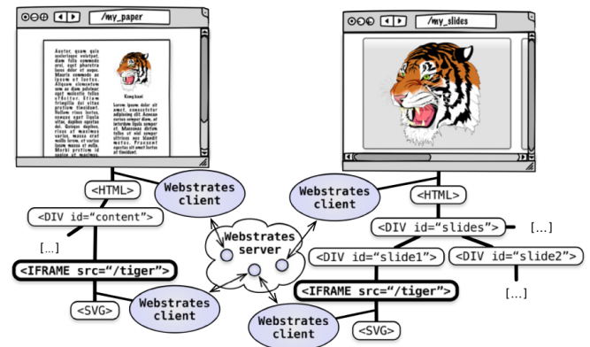
Figure 2: Two webstrates transclude the same image webstrate. Changes in the figure appear immediately in both windows. Reprinted from [16].
