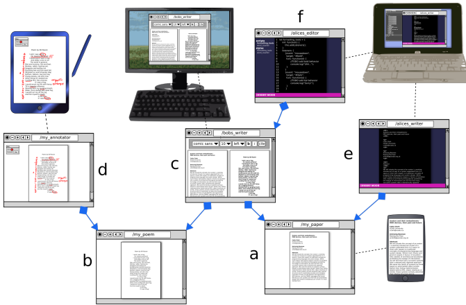
Figure 3: An example of a network of interconnected webstrates. The blue arrows are transclusions establishing application-document relationships. a) A paper, displayed on a mobile device. b) A poem. c) Bob’s word processor editing a and b on his desktop computer. d) Bob’s annotation webstrate which lets Bob hand-annotate webstrates with his tablet and stylus. e) Alice’s HTML markup editor, editing the paper a on her laptop. f) Alice’s script editor, extending Bob’s word processor on a different window of her laptop.
